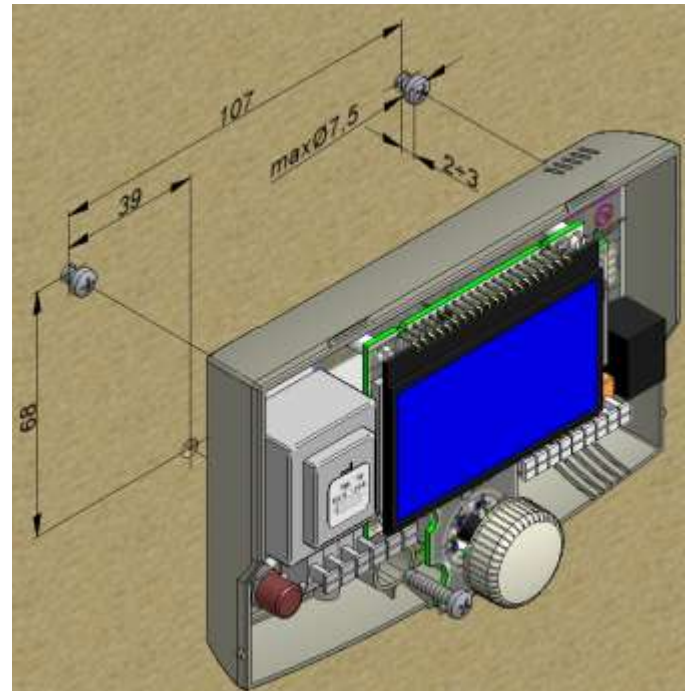
Fig. 8.2 Installing the regulator on a wall (reference drawing)
