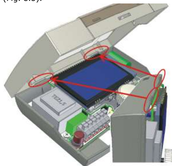
Fig. 8.5 Closing the casing - step one (reference drawing)
