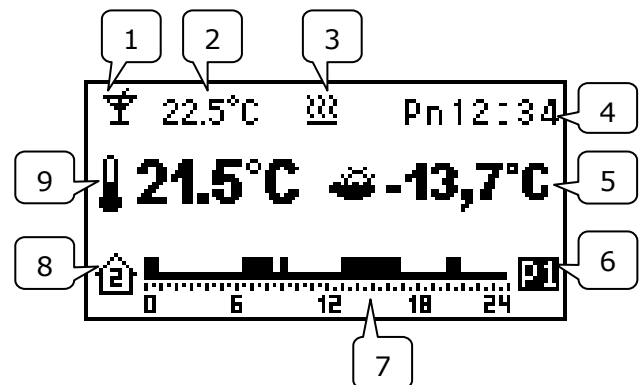
Fig. 7.1 Exemplary view of the main screen for thermostat 2
