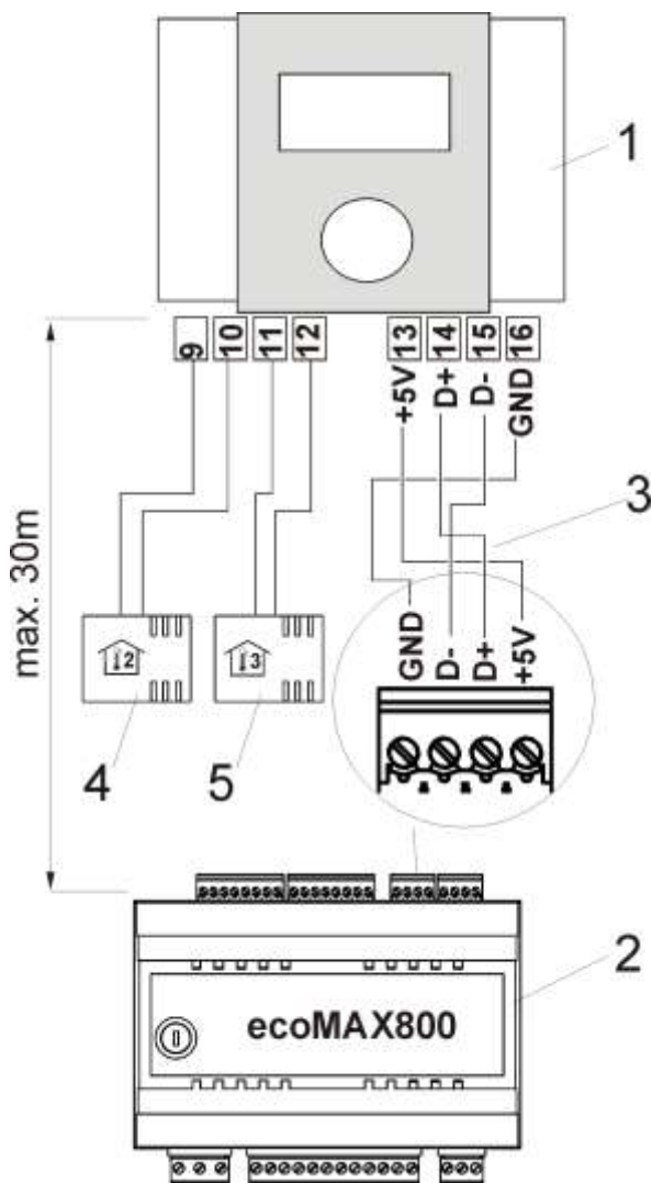
Fig. 8.3 Electrical diagram, where: 1 - ecoSTER 200 room panel, 2 - ecoMAX800 R or T regulator, 3 - connecting cable, 4 - room sensor of thermostat 2 type CT7, 5 - room sensor of thermostat 3 type CT7.
